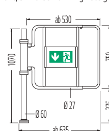
N exit, swivel barrier in high design
