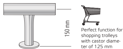
Collision height for shopping trolleys
